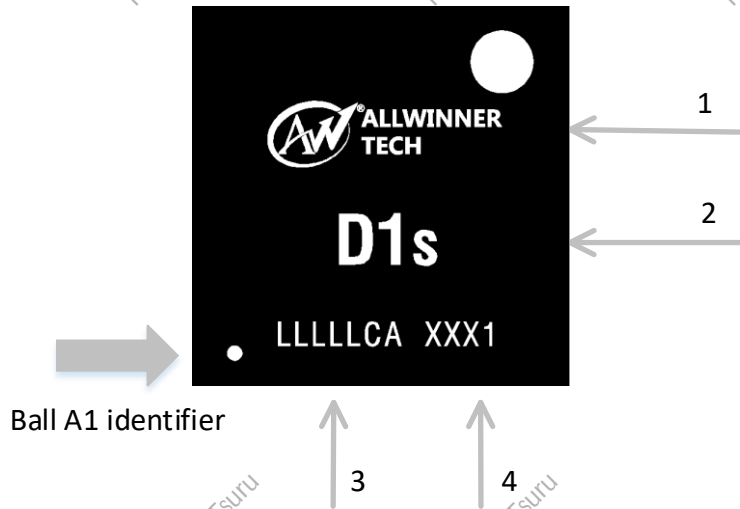
Figure 11-1 D1s Marking
