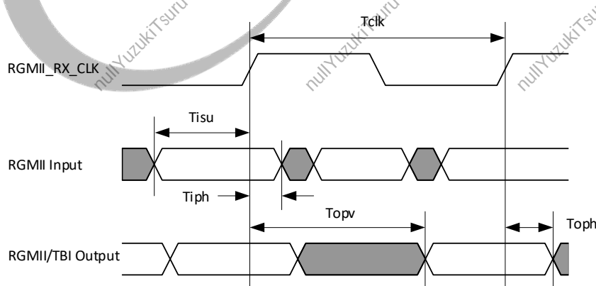
Figure 5-12 RGMII Interface Receive Timing
