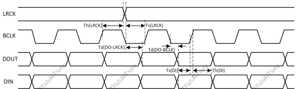
Figure 5-24 I2S/PCM Timing in Slave Mode
